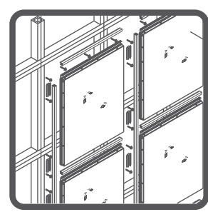
Tray Panel with Clip
