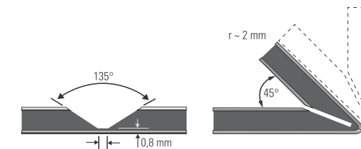
135° V-groove for folds up to 135°
