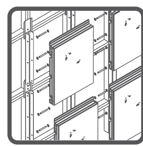
Hook-on
