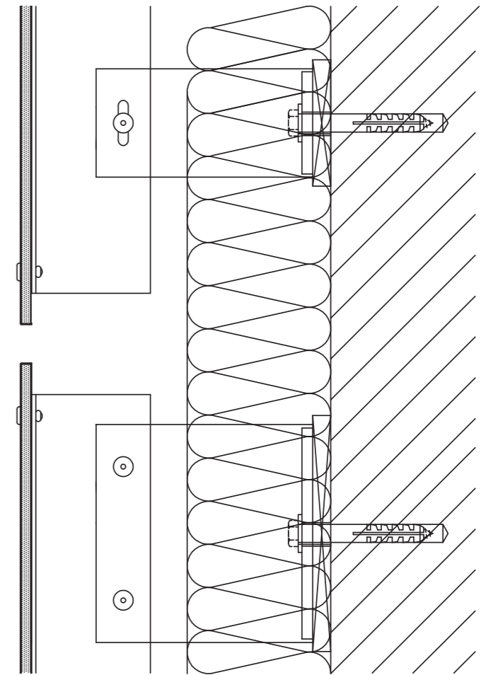
Vertical Section
