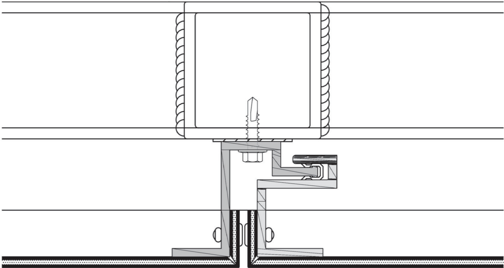
Joint Section
