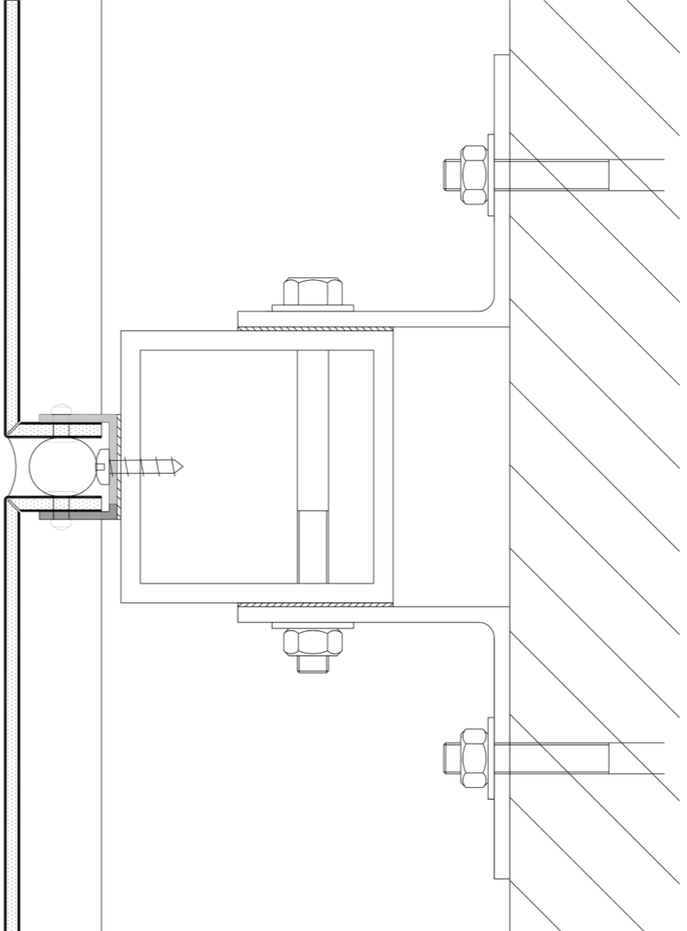
Vertical Section
